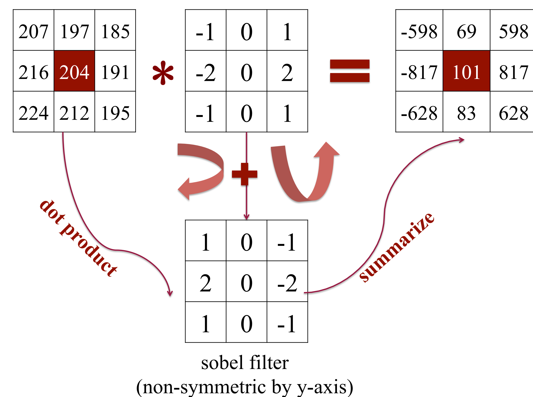
Figure 2: Convolution process
